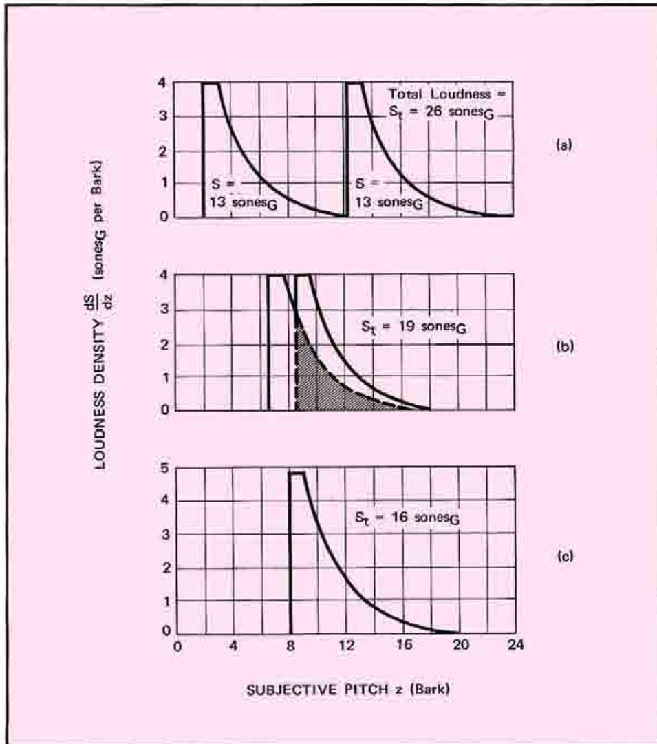
Figure 6. Effect of masking when two sounds are widely spaced in frequency (a), when their masking curves overlap (b), and when both sounds fall in the same critical band but are incoherent (c).
